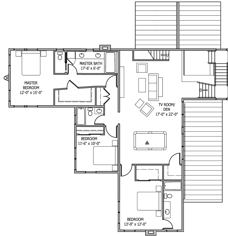
SECOND FLOOR PLAN - OPTION 2
