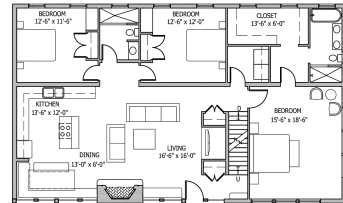
ENTRY LEVEL PLAN
