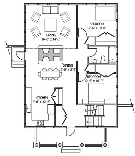
ENTRY LEVEL OPTION 1
